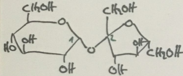
Sucrose
