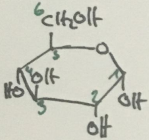
\alpha -D-Glucose
