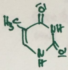
Thymin
